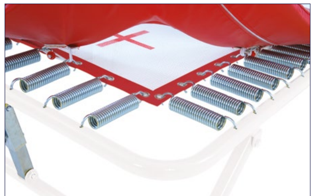
34 galvanized springs connected to the PVC bed
